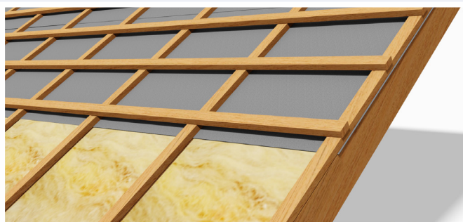
Draped over rafters - fully supported warm roof
